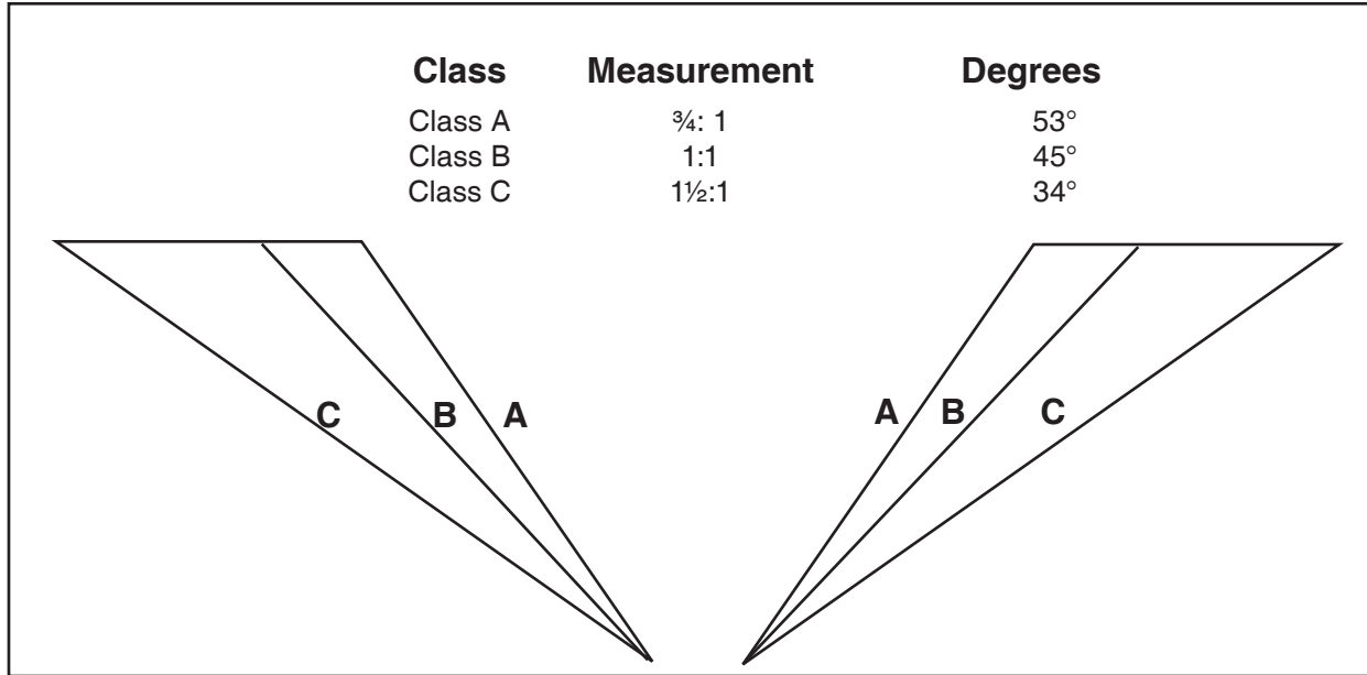
Simple Slope Excavation
