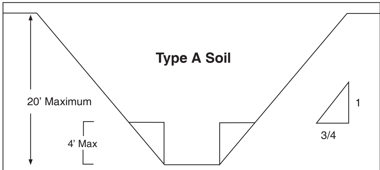
Simple Bench Excavation
